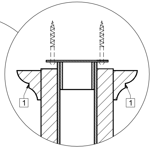
DETAILED SECTION VIEW
