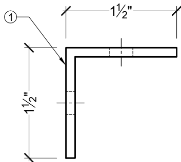
4 - ALUMINUM PREPUNCHED BRACKETS
